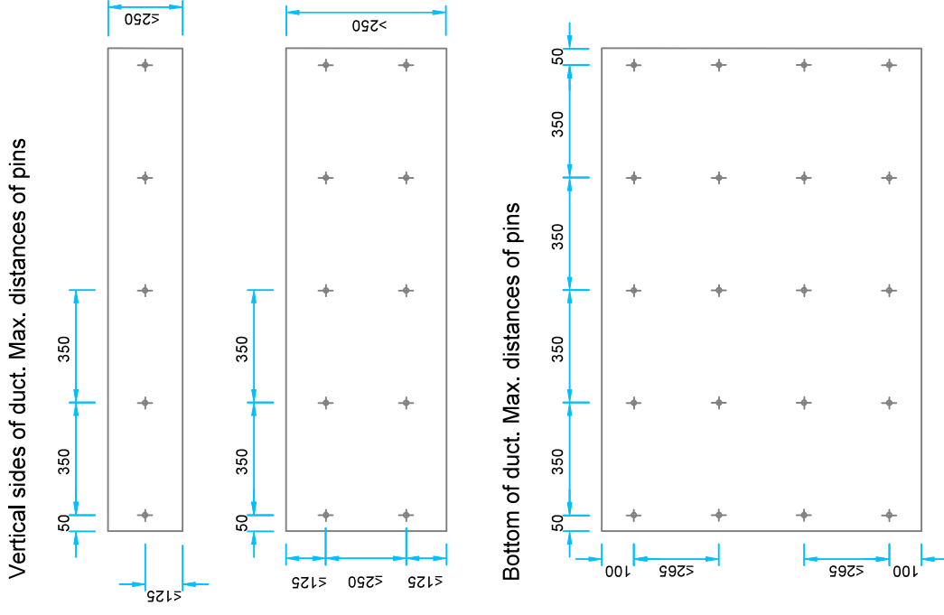
Figure 14 (2/2). Rectangular horizontal duct, insulation CONLIT Fire Board EI60, fire resistance class EI 60: arrangement of steel pins
