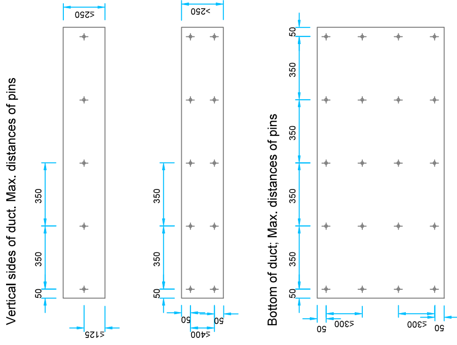
Figure 18 (2/2). Rectangular horizontal duct, insulation CONLIT Fire Board EI120, fire resistance class 120: arrangement of steel pins
