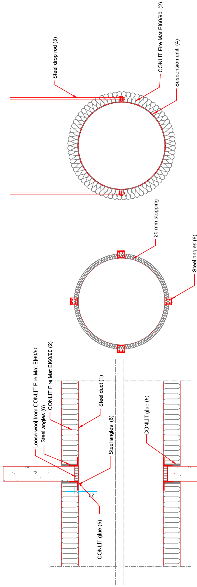
Figure 3: Circular horizontal duct, insulation CONLIT Fire Mat EI60/90, fire resistance class EI 60
