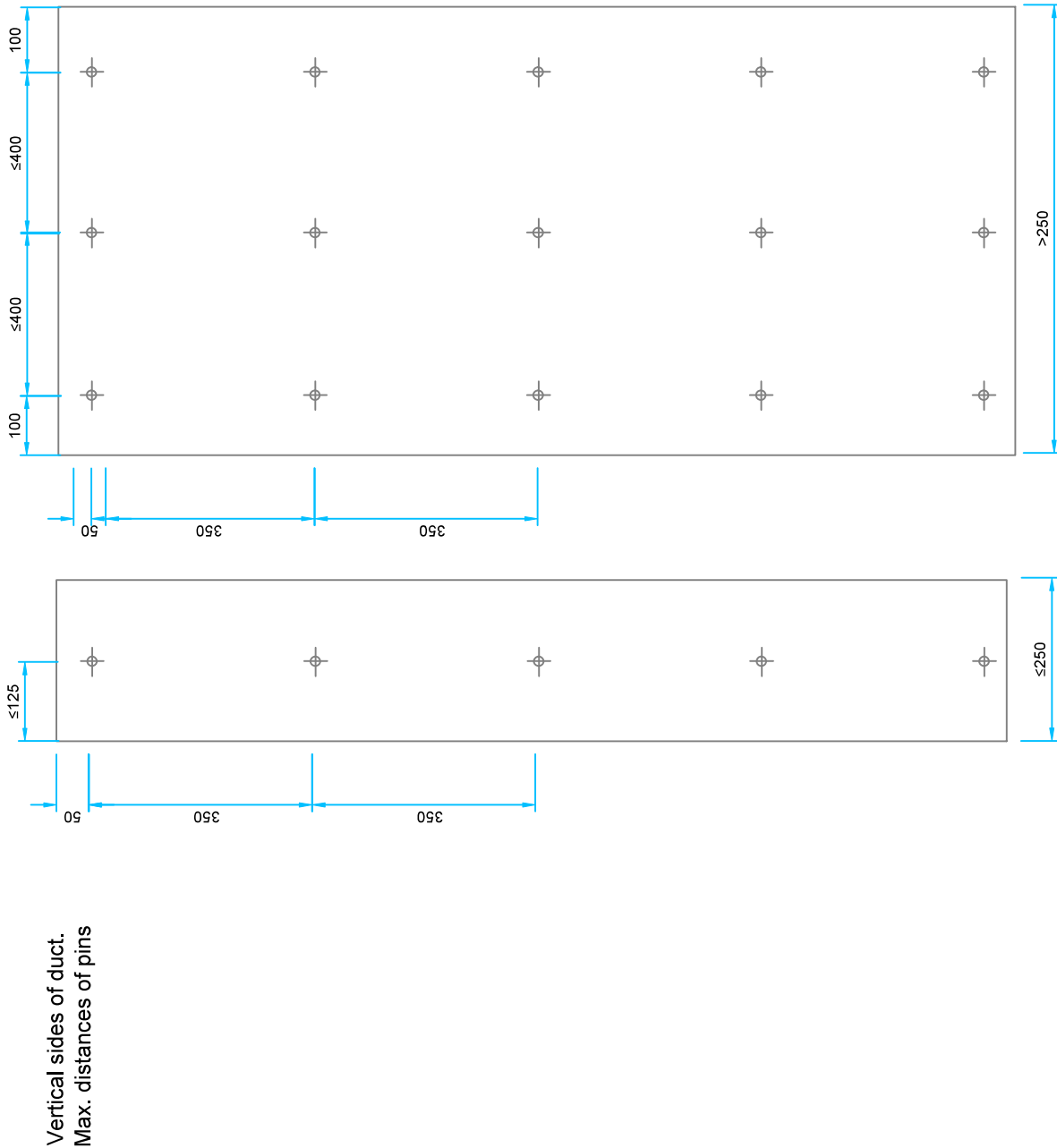
Figure 19 (2/2). Rectangular vertical duct, insulation CONLIT Fire Board EI120, fire resistance class EI 120
