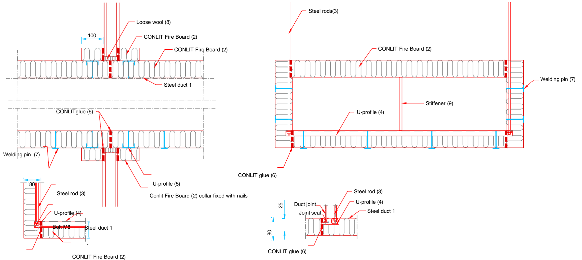
Figure 16 (1/2). Rectangular horizontal duct, insulation CONLIT Fire Board EI90, fire resistance class EI 90
