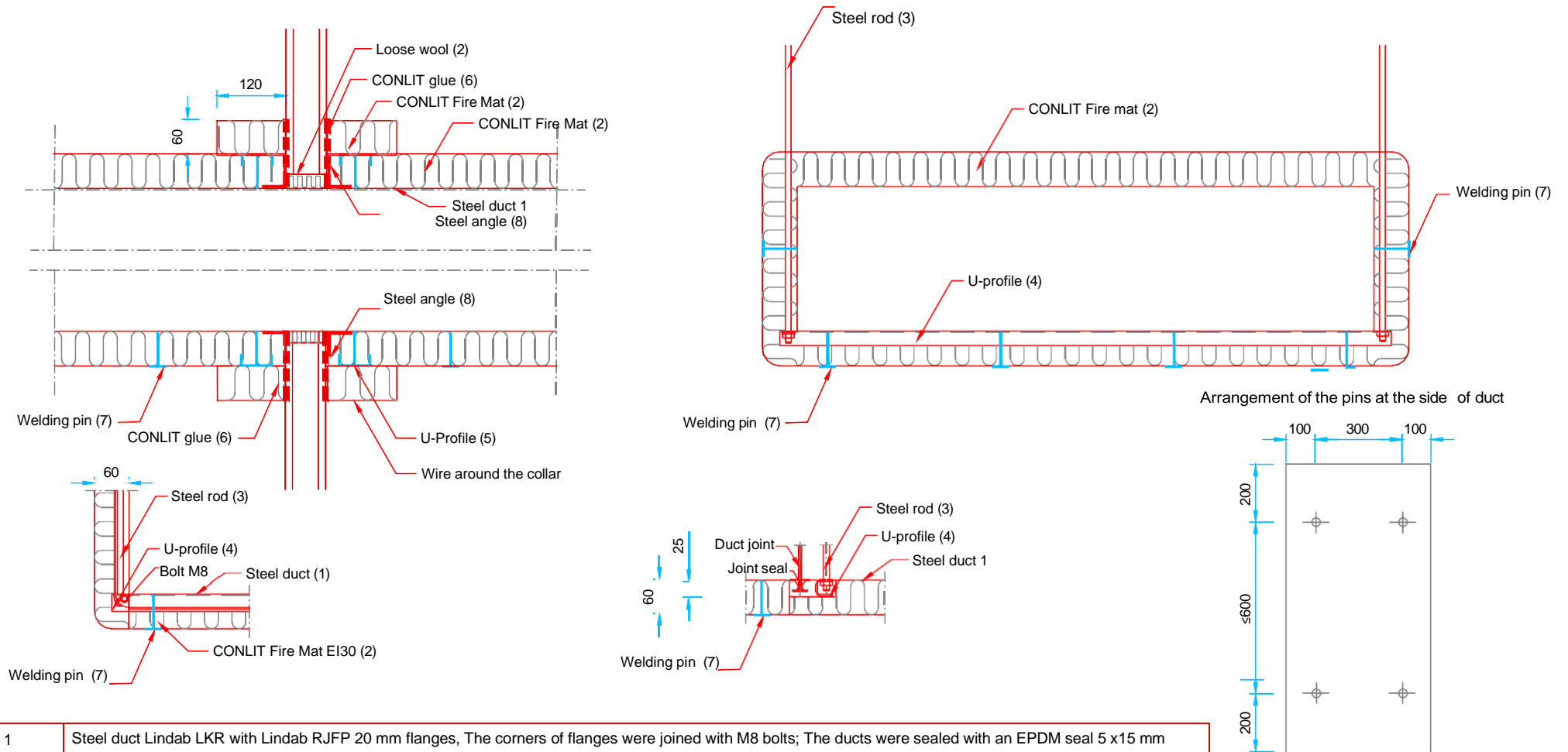
Figure 10. Rectangular horizontal duct, CONLIT Fire Mat EI30, fire resistance class EI 30
