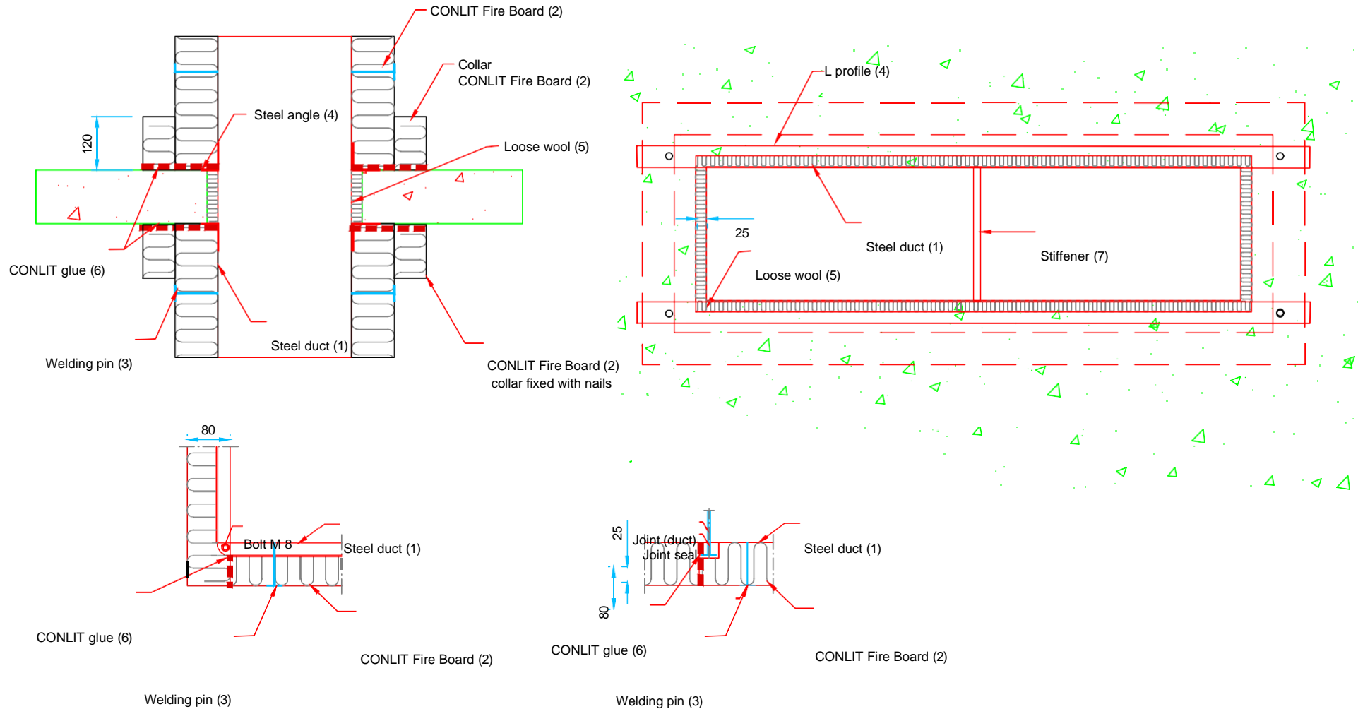
Figure 17 (1/2). Rectangular vertical duct, insulation CONLIT Fire Board EI90, fire resistance class EI 90
