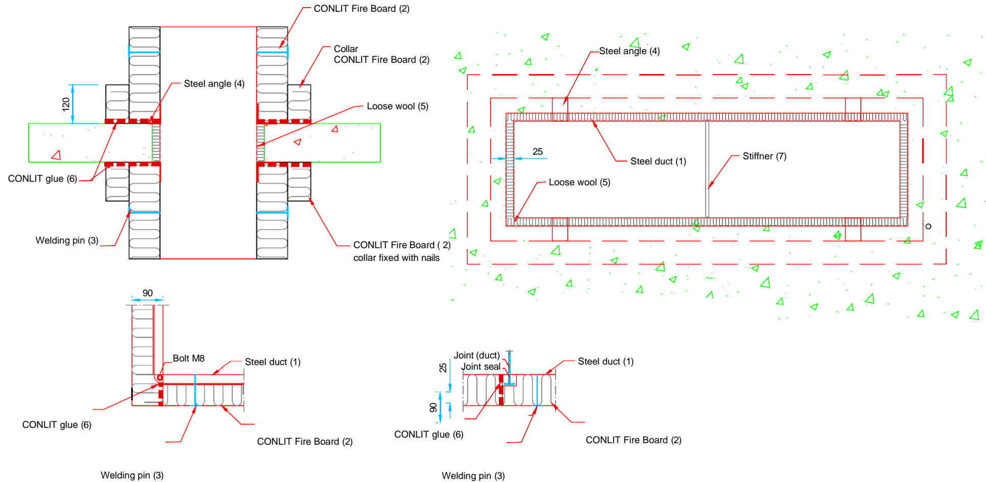
Figure 19 (1/2). Rectangular vertical duct, insulation CONLIT Fire Board EI120, fire resistance class EI 120
