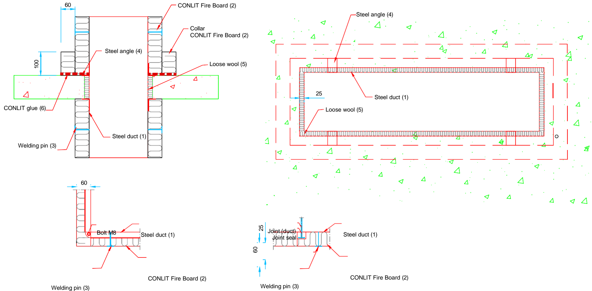
Figure 13 (1/2). Rectangular vertical duct, insulation CONLIT Fire Board EI30, fire resistance class EI 30
