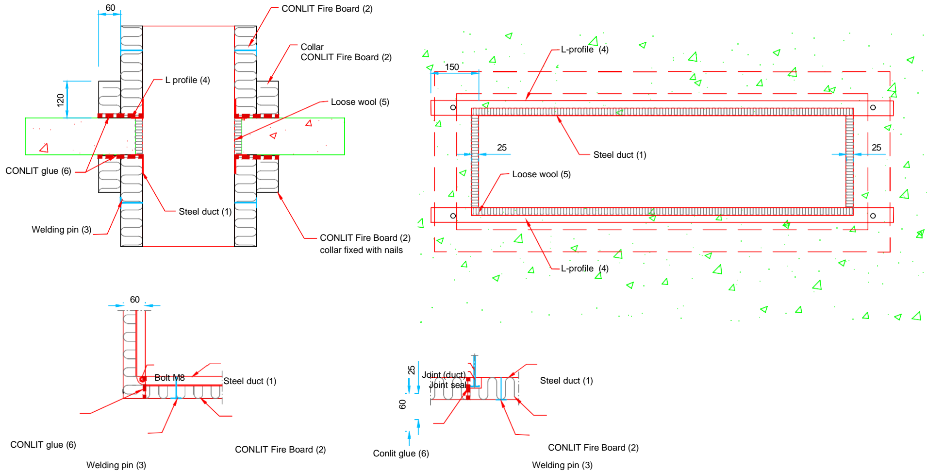
Figure 15 (1/2). Rectangular vertical duct, insulation CONLIT Fire Board EI60, fire resistance class EI 60
