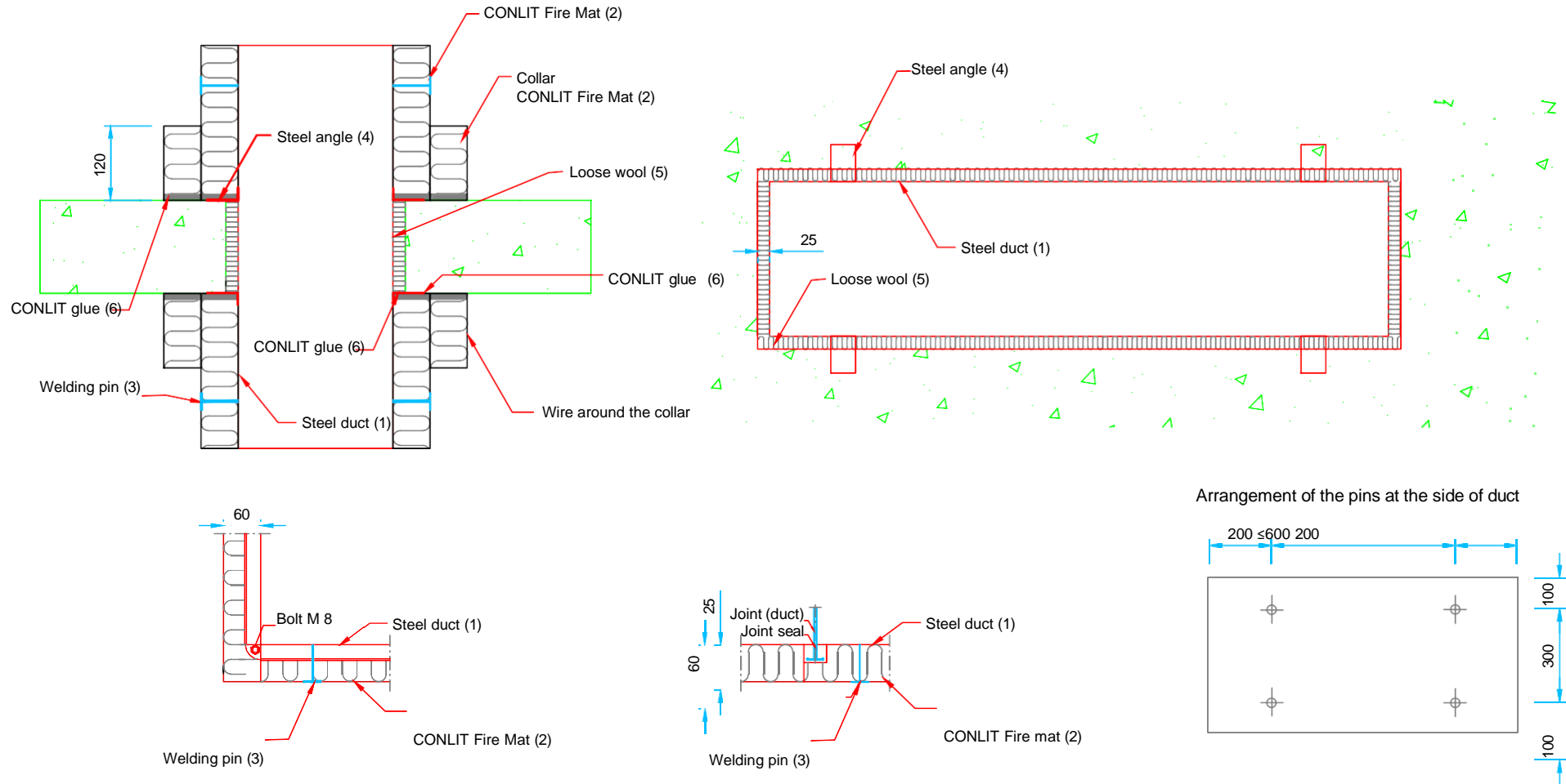
Figure 11. Rectangular vertical duct, insulation CONLIT Fire Mat EI30, fire resistance class EI 30
