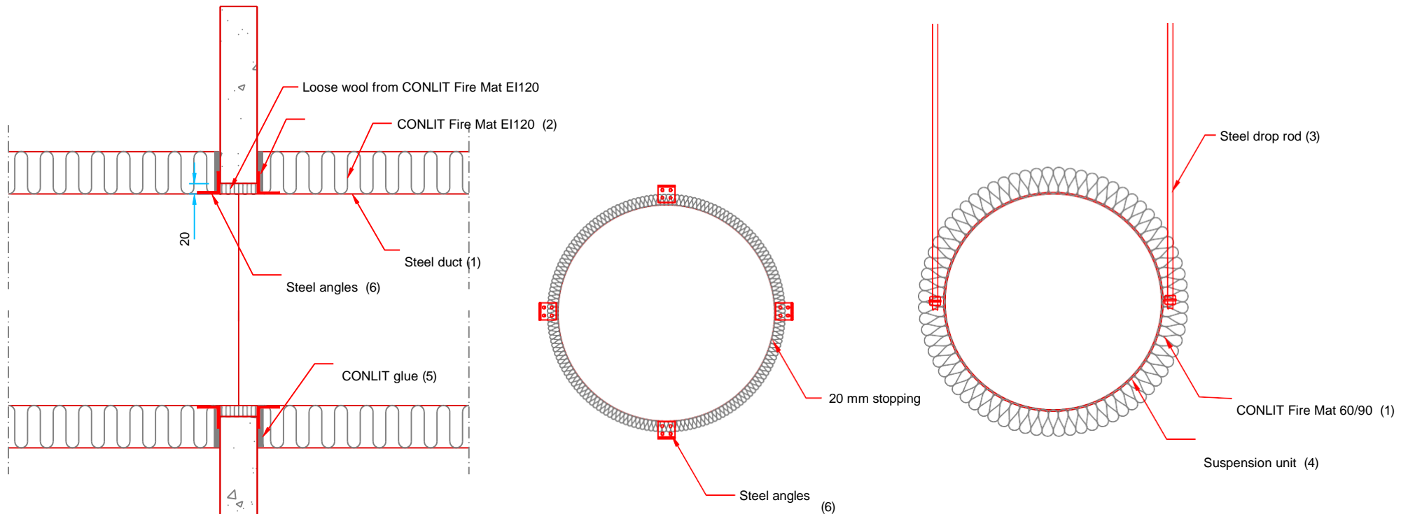
Figure 7: Circular horizontal duct, insulation CONLIT Fire Mat EI120, fire resistance class EI 120
