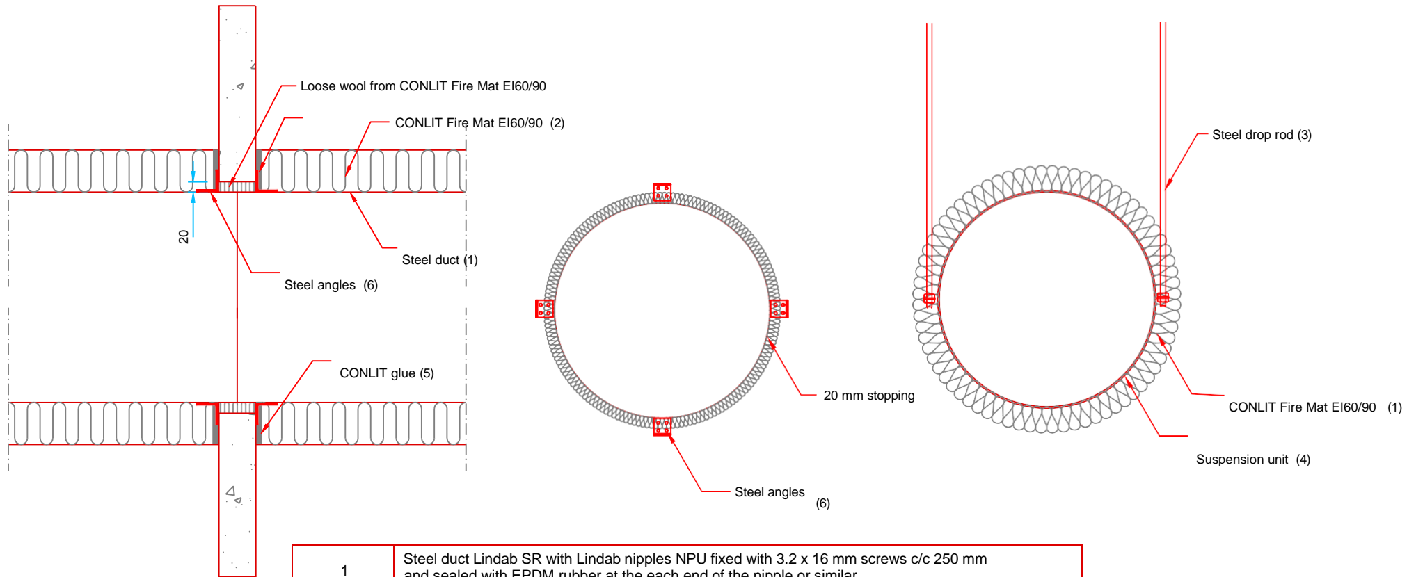
Figure 5: Circular horizontal duct, insulation CONLIT Fire Mat EI60/90, fire resistance class EI 90
