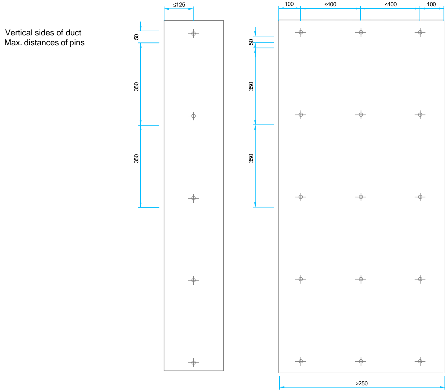
Figure 17 (2/2). Rectangular vertical duct, insulation CONLIT Fire Board EI90, fire resistance class EI 90: arrangement of steel pins
