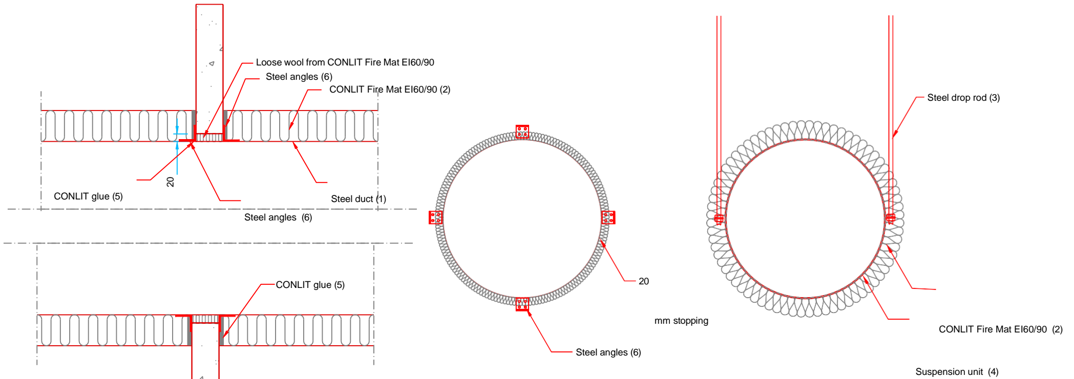
Figure 3: Circular horizontal duct, insulation CONLIT Fire Mat EI60 and CONLIT Fire Mat EI60/90, fire resistance class EI 60
