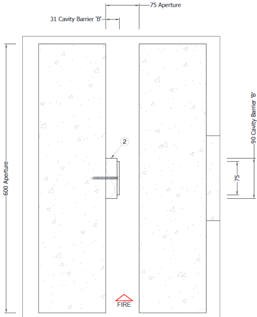
Figure PAR/25141/02:01 – Test report WF407778 Cavity barrier B in aperture 75mm wide. Cavity barrier B has no hanging bracket but is directly screwed to wall
