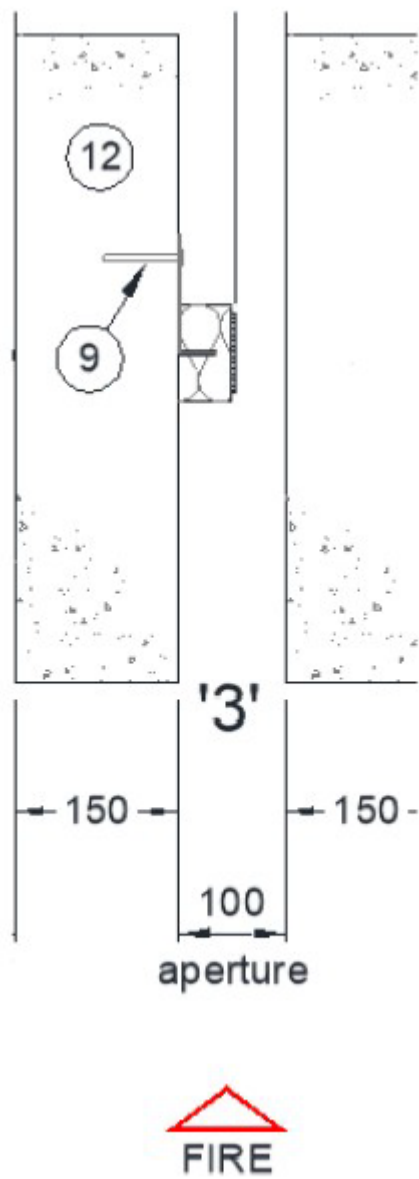
Figure PAR/25141/02:02 – Test report WF397020 Specimen 3 in a 100mm wide aperture
